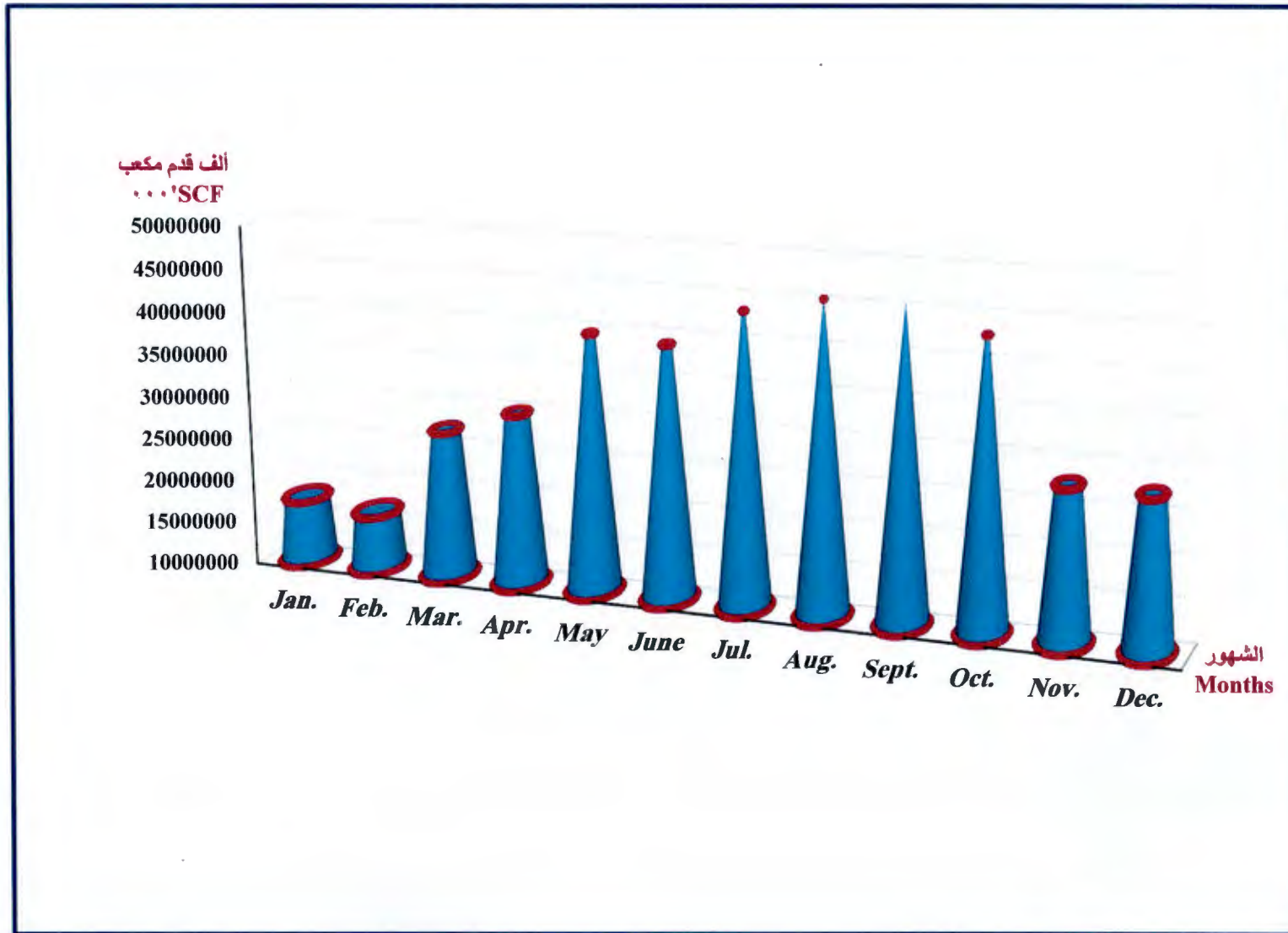
Consumption of Natural Gas By Power & Distillation Plants ('000 SCF) During 2018
